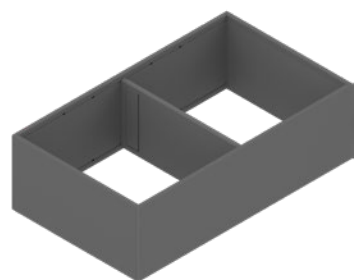
High frame (long) Width 218 mm Length 370 mm Height 110 mm
