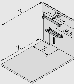
Drilling distances – cabinet base | cross member
